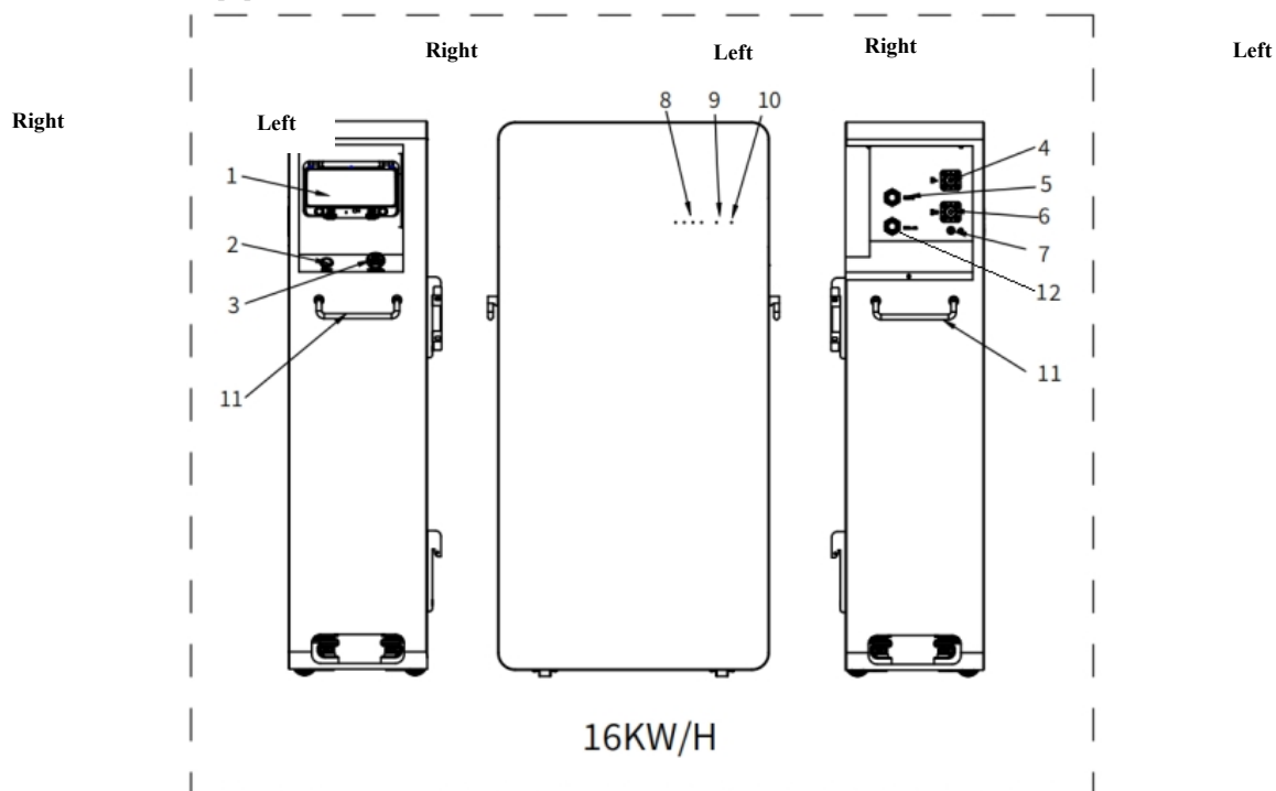
Figure 2-3 Battery Appearance
